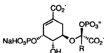
3a R = \text{CH}_2\text{F} R-3b R = \text{CHF}_2 K_{i(\text{app})} = 4 \pm 0.3 \text{ nM} R-3c R = \text{CF}_3 K_{i(\text{app})} = 32 \pm 3 \text{ nM}
