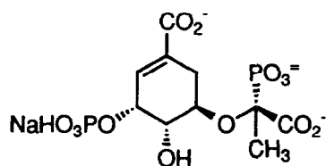
R-2 K_{i(\text{app})} = 5 \pm 1 \text{ nM}
