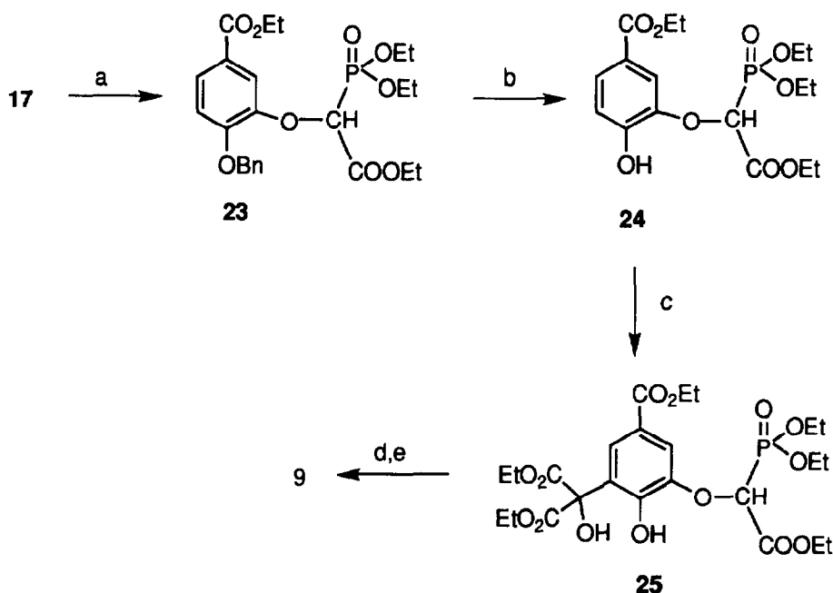
Scheme 4. Reagents and conditions: (a) \text{Et}_2\text{O}_3\text{PC}(=\text{N}_2)\text{CO}_2\text{Et} , \text{Rh}_2(\text{OAc})_4 , benzene, reflux (68%); (b) \text{H}_2 , 10% Pd/C, EtOH, 50 psi (95%); (c) DEKM, \text{SnCl}_4 , \text{CH}_2\text{Cl}_2 , 0 °C to room temperature, 36 h (30%); (d) \text{TMSBr} , \text{C}_5\text{H}_5\text{N} , \text{CH}_2\text{Cl}_2 ; (e) \text{NaOH} , \text{H}_2\text{O} ; DEAE Sephadex chromatography (20%).
