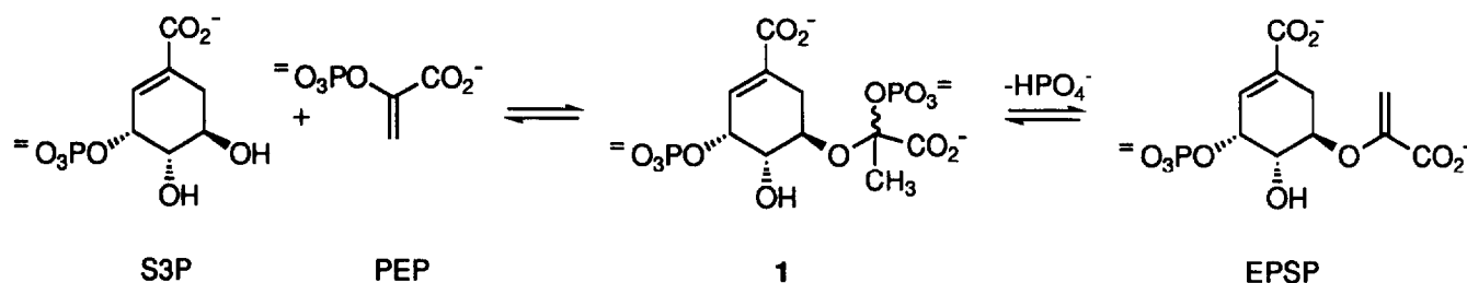
Scheme 1. The reaction catalyzed by EPSP synthase.
