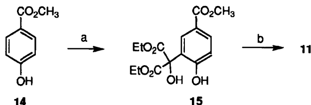
Scheme 2. Reagents and conditions: (a) DEKM, \text{SnCl}_4 , \text{CH}_2\text{Cl}_2 , 0^\circ\text{C} to room temperature, 36 h (80%); (b) \text{NaOH} , \text{H}_2\text{O} ; DEAE Sephadex chromatography.
