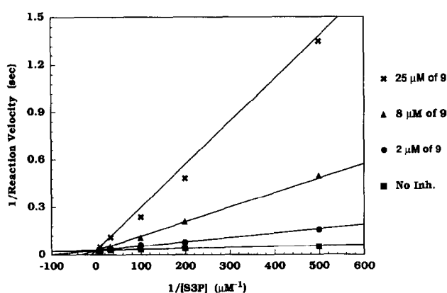
Figure 4. Inhibition of EPSP synthase by compound 9 . Double reciprocal plot of reaction velocity versus S3P concentration obtained at varying concentration of inhibitor 9 . The lines drawn were obtained from a nonlinear least-squares fit to the observed data using eq. (1) which corresponds to a kinetic model for competitive inhibition. Fitting to eq. (2), corresponding to a kinetic model for mixed inhibition, gave a very poor fit. The data, therefore, is best interpreted in terms of competitive inhibition versus S3P.
