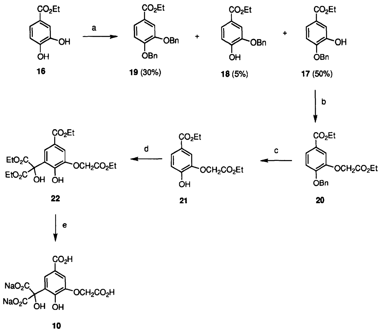
Scheme 3. Reagents and conditions: (a) BnBr, K 2 CO 3 , 2-butanone, 5 h, reflux; (b) ICH 2 CO 2 Et, K 2 CO 3 , acetone, 25 h, reflux (80%); (c) H 2 , 10% Pd/C, EtOH, 50 psi, (75%); (d) DEKM, SnCl 4 , CH 2 Cl 2 , 0 °C to room temperature, 36 h (56%); (e) NaOH, THF (85%).
