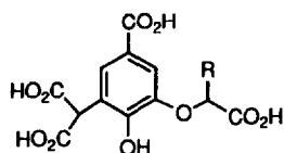
13a R = -\text{PO}_3\text{H}_2 13b R = -\text{H}
