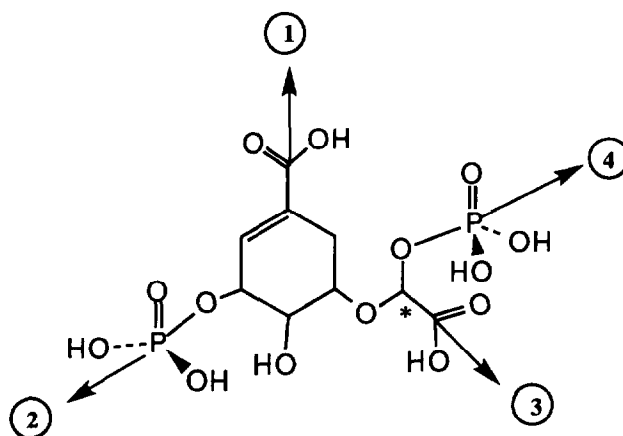
Figure 1. The pharmacophore starting point for modeling compound 1 with Sybyl. Dummy atoms (1–4) were symmetrically positioned 3 Å away from the center atom in each of the anionic functional groups.
